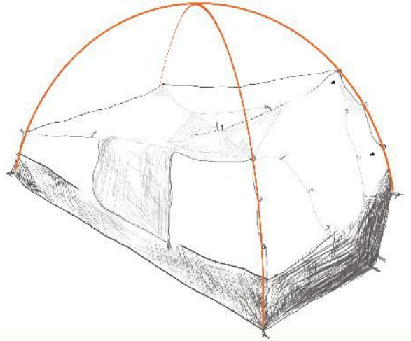
2 Attach the orange cross poles (longer two poles)
